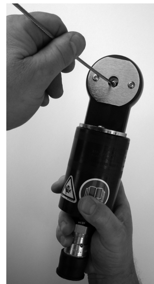
610 Portable Swager for use with 1/8" and 3/16" diameter cable.
