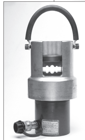
< Model 650 Swager for 1/8" through 3/8" cable.
